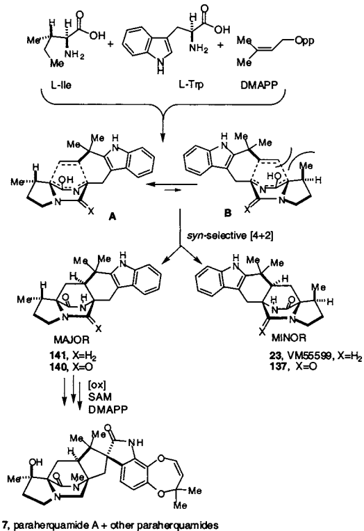
Scheme 24. Unified Biogenesis of the Paraherquamides and VM55599 38
