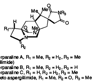
FIGURE 3. Structures of the asperparalines.
