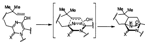
Scheme 1. Proposed Diels–Alder Reaction Forming the Core Structure of the Brevianamides, Paraherquamides, and Asperparalines
