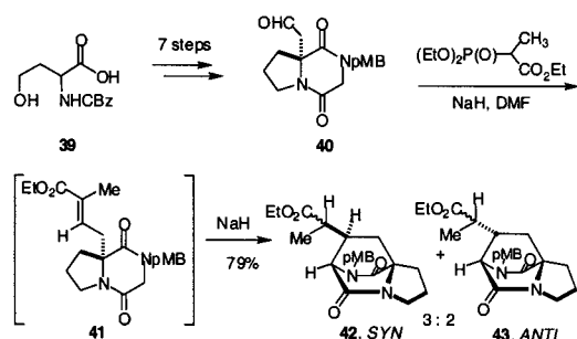
Scheme 5. Initial S_N2' Cyclization Model Studies on the Brevianamides 20
