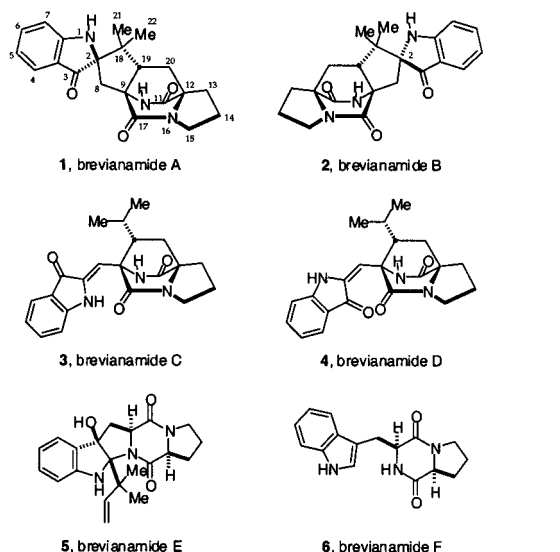
FIGURE 1. Structures of the brevianamides.
