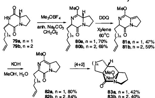
Scheme 14. Model Intramolecular Diels–Alder Cycloadditions 27
